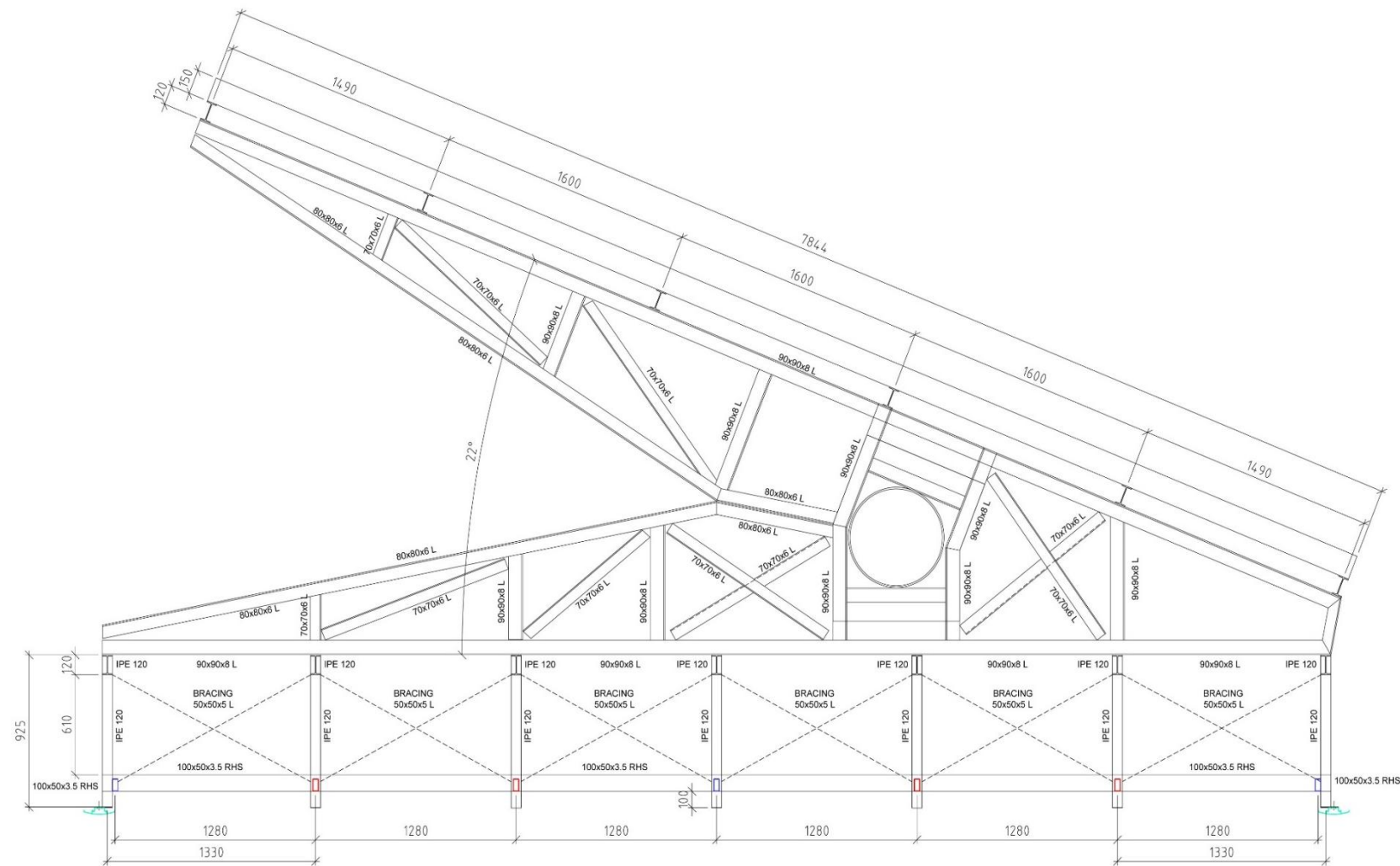
PLAN ON TYPICAL HORIZONTAL TRUSS SCALE 1:25
